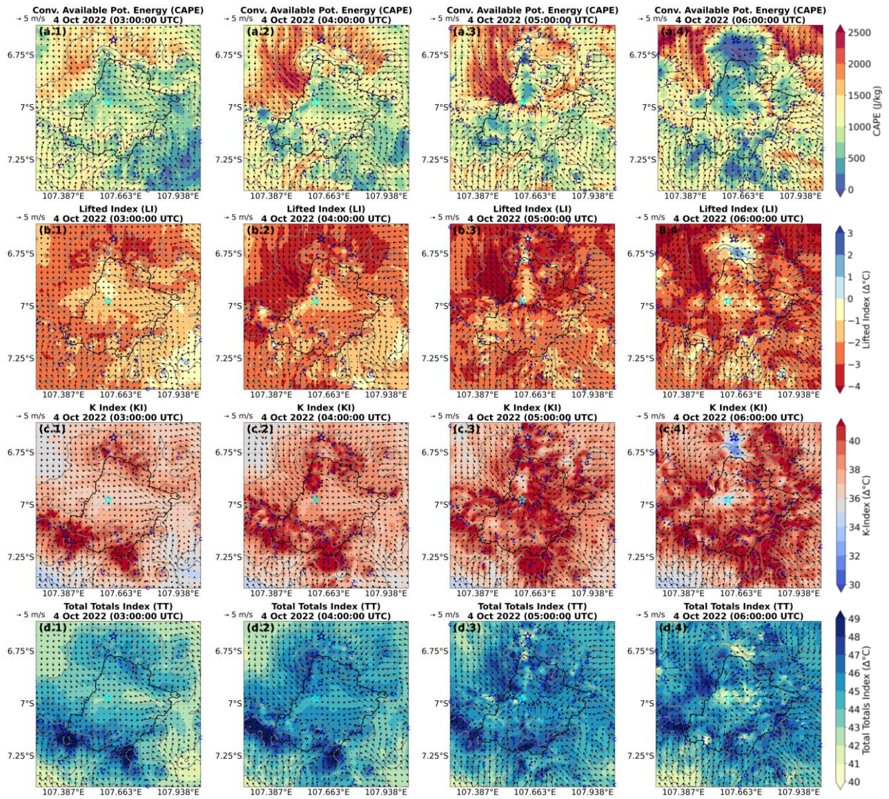
Figure 3. Spatial distribution of stability indices over the Bandung Basin: (a) CAPE, (b) LI, (c) KI, (d) TT ( ^{\circ}\text{C} , shaded), with the wind vector at the lowest level of the model ( \sim 25 m) and convergence zones (divergence \leq -0.0035 \text{ s}^{-1} , blue C symbols). Black contours indicate the Bandung Basin boundaries. Dark blue and cyan stars mark representative points of convective cells in north mountain region and valley (Pagarsih region), respectively.
